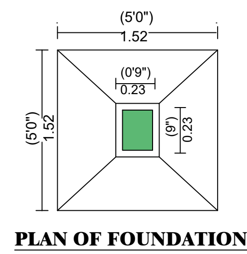
PLAN OF FOUNDATION
