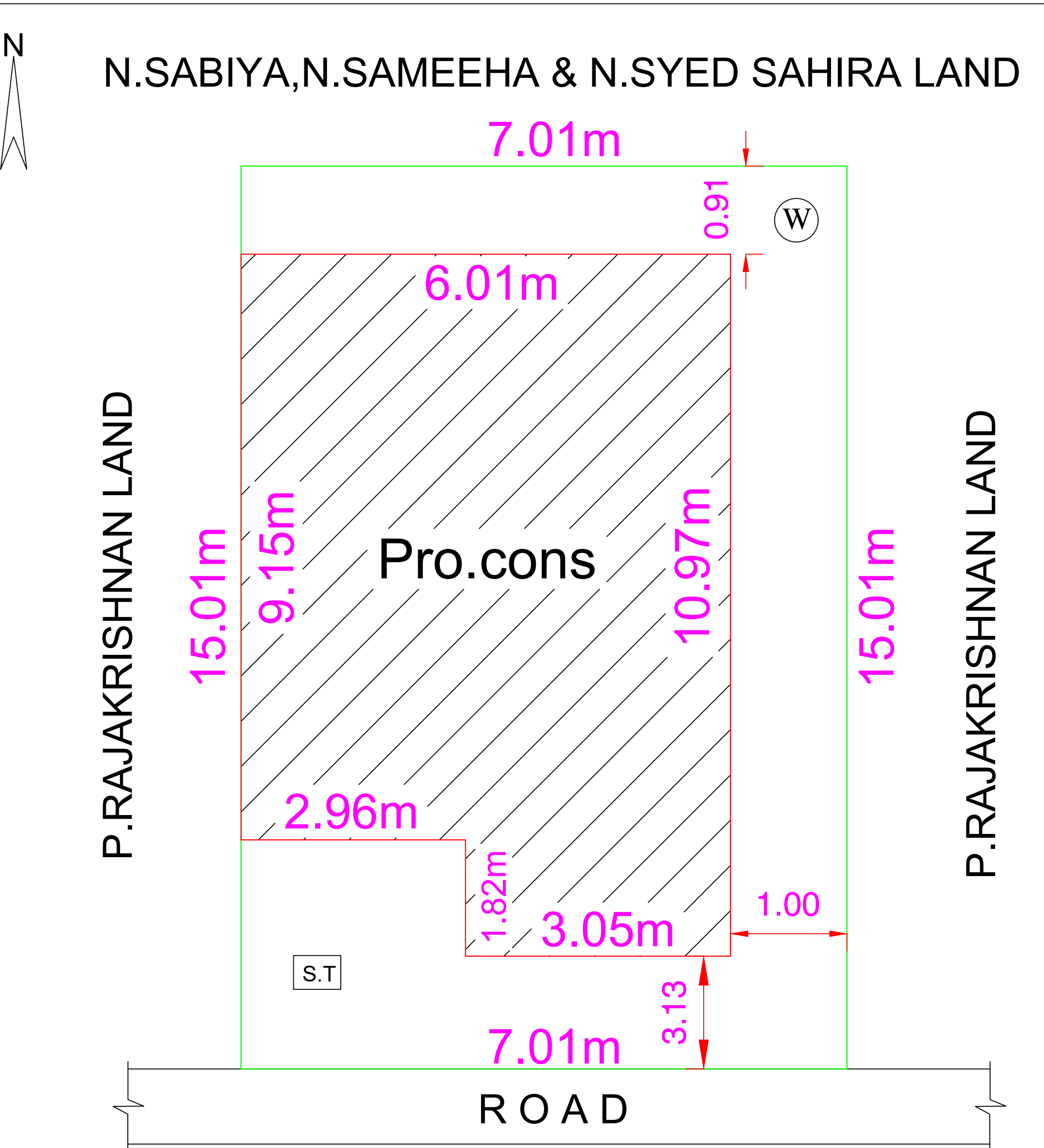
SITE PLAN
