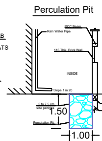
Percolation Pit
