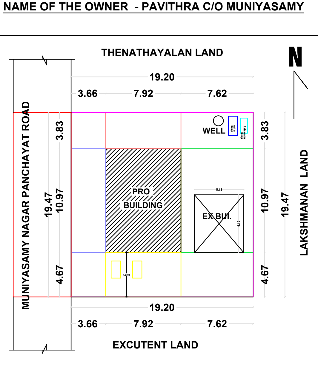
SITE PLAN & KEY PLAN
