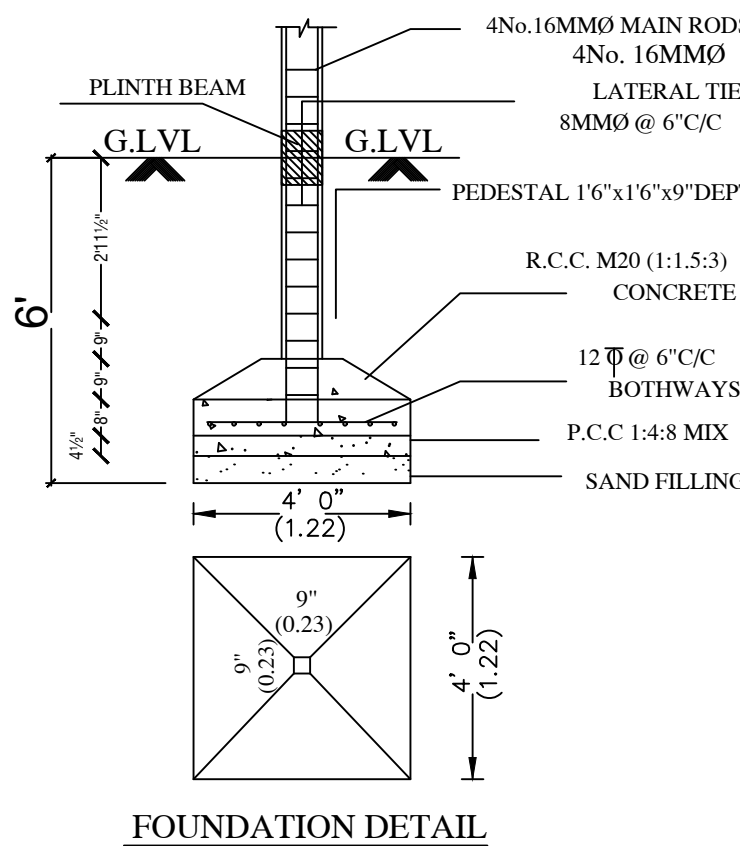
FOUNDATION DETAIL
