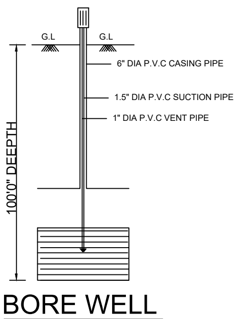
BORE WELL
