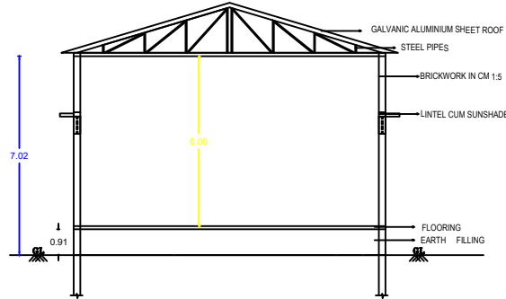
SECTION ON-AB
