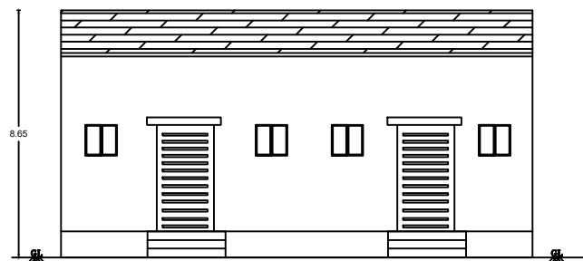
FRONT ELEVATION
