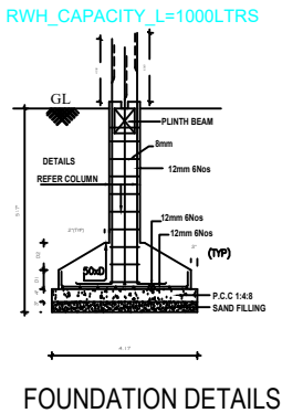
FOUNDATION DETAILS
