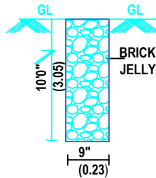
PERCULATION PIT
