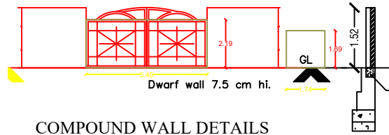
COMPOUND WALL DETAILS
