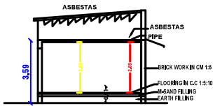
SECTION
