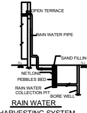
RAIN WATER HARVESTING SYSTEM
