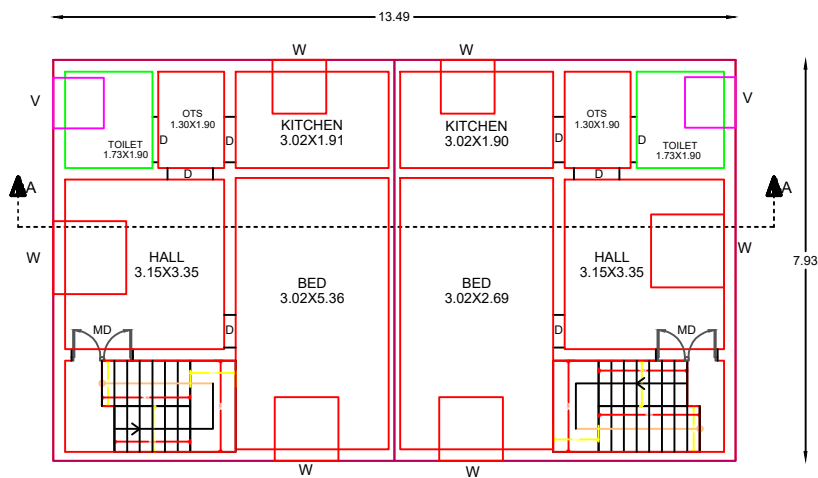
PROPOSED RESIDENTIAL GROUND FLOOR PLAN
