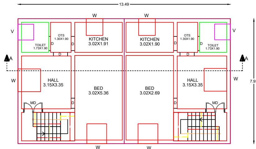
PROPOSED RESIDENTIAL FIRST FLOOR PLAN
