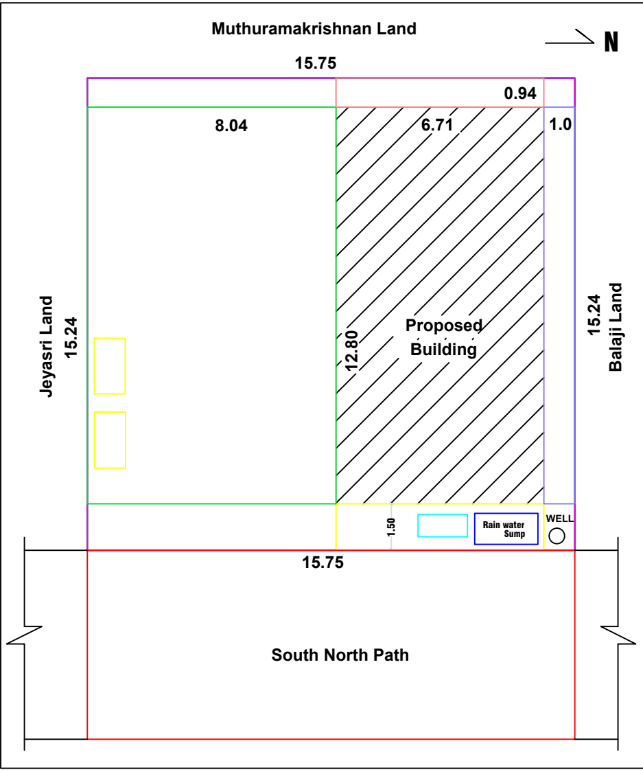
SITE PLAN CUM KEYPLAN
