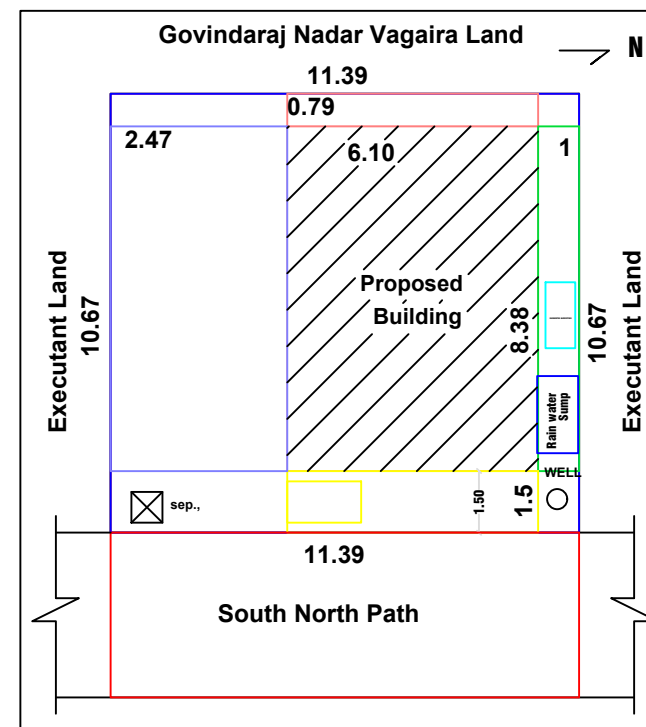
SITE PLAN CUM KEYPLAN
