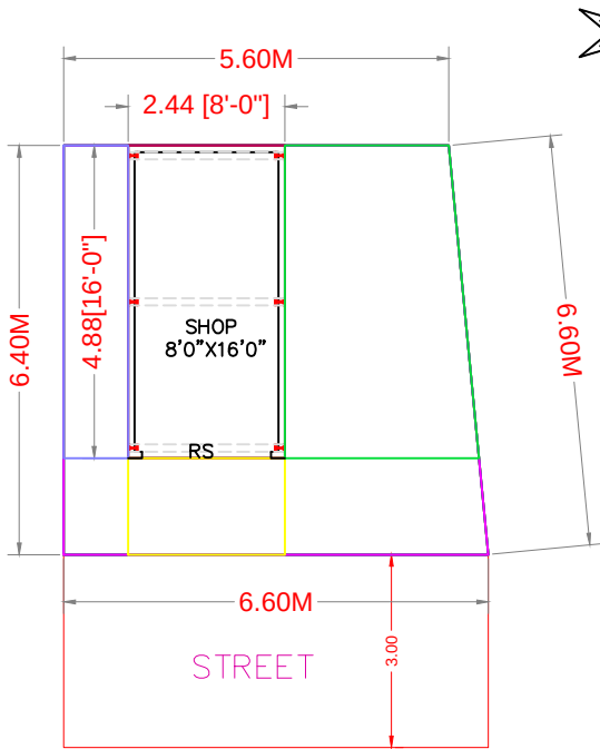
SITE CUM GROUND FLOOR
