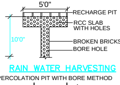
RAIN WATER HARVESTING PLAN
