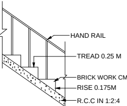
STAIRCASE DETAIL
