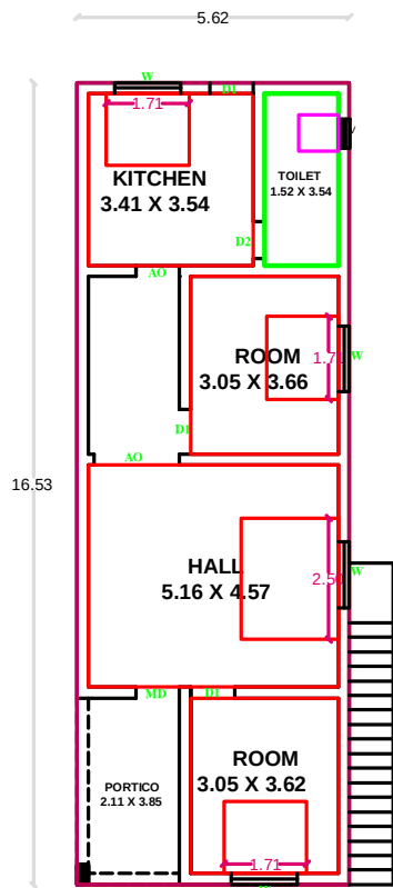
GROUND FLOOR PLAN PROPOSED
