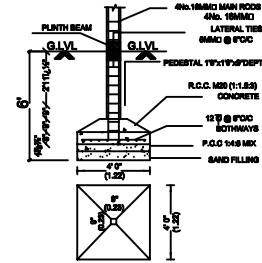
FOUNDATION DETAIL
