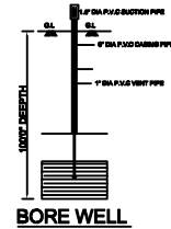
BORE WELL
