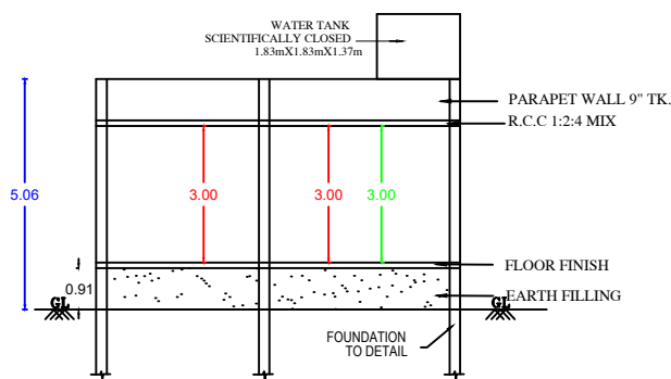
SECTION AB
