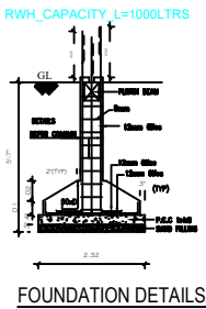
FOUNDATION DETAILS
