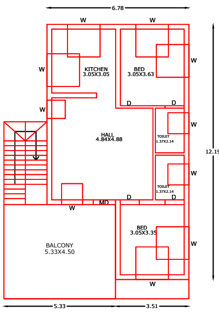
PROPOSED RESIDENTIAL FIRST FLOOR PLAN
