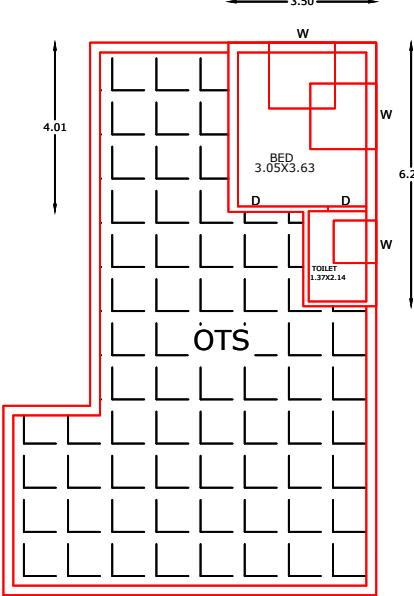
PROPOSED RESIDENTIAL SECOND FLOOR PLAN
