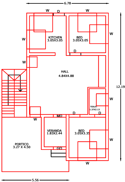
EXISTING RESIDENTIAL GROUND FLOOR PLAN
