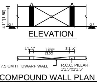
COMPOUND WALL PLAN
