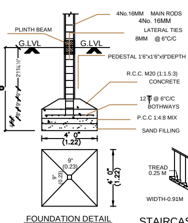
FOUNDATION DETAIL
