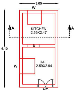
PROPOSED RESIDENTIAL GROUND FLOOR PLAN
