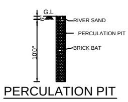
FOUNDATION DETAIL
