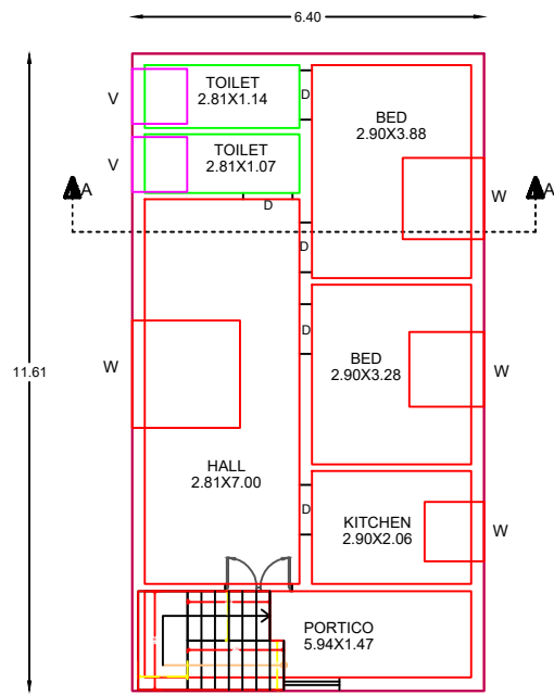
PROPOSED RESIDENTIAL GROUND FLOOR PLAN
