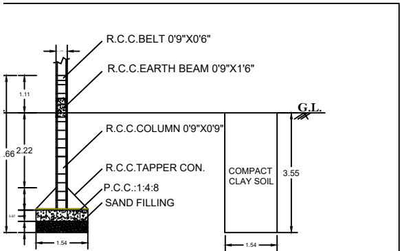
FOUNDATION DETAILS-MIDDLE COLUMN
