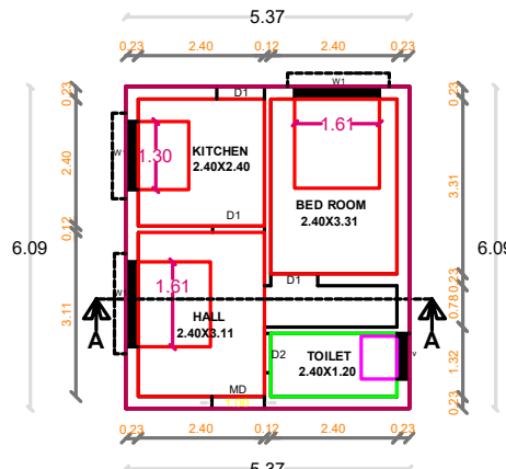
GROUND FLOOR PLAN PROPOSED
