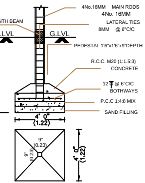
FOUNDATION DETAIL
