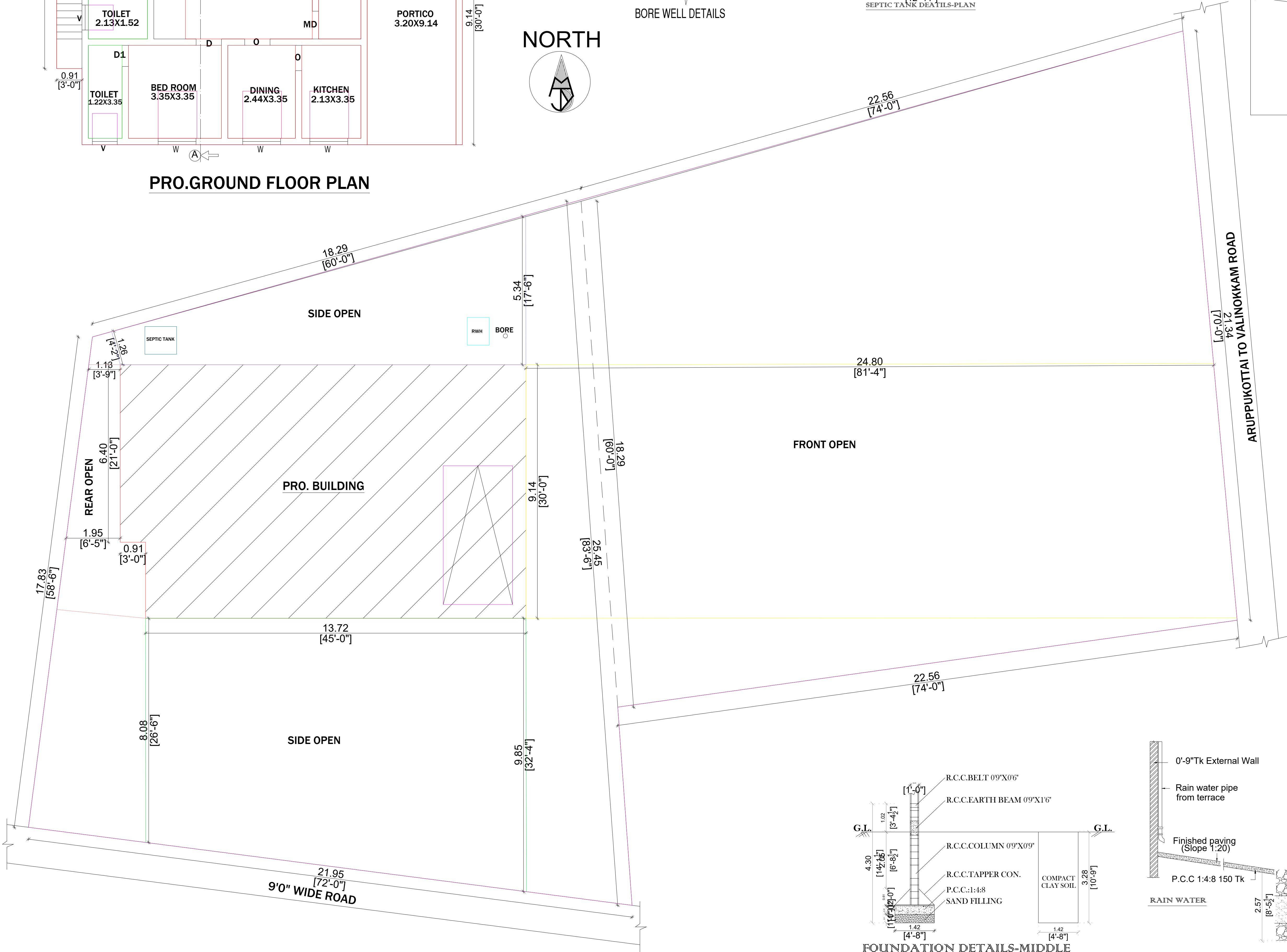
SITE PLAN
