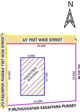
SITE PLAN
