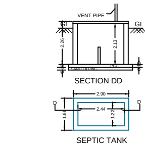
SEPTIC TANK
