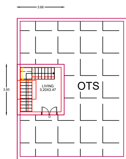
PROPOSED RESIDENTIAL FIRST FLOOR & TERRACE PLAN
