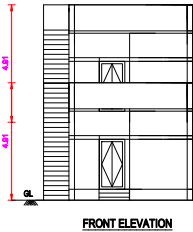
FRONT ELEVATION
