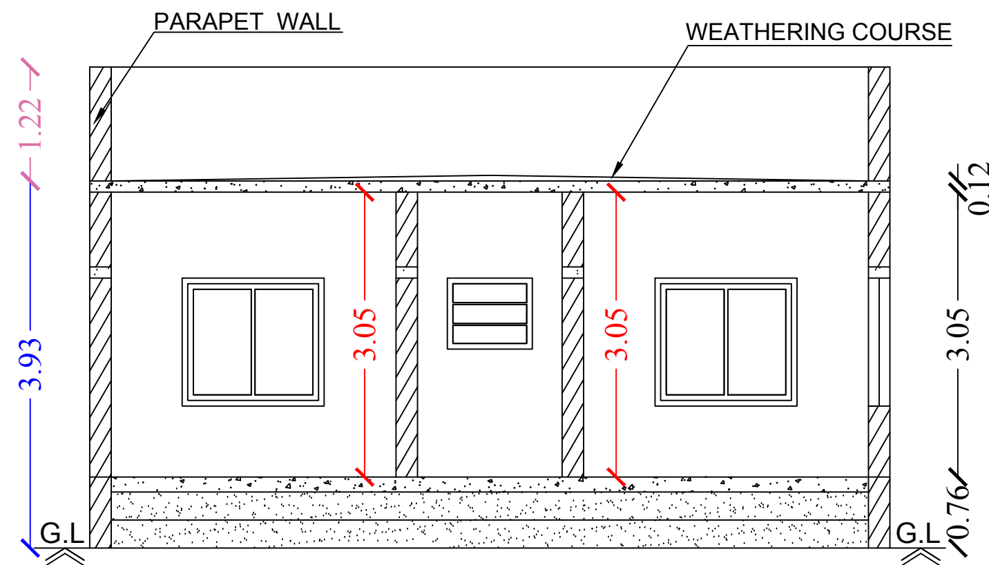
Section on-"AA"
