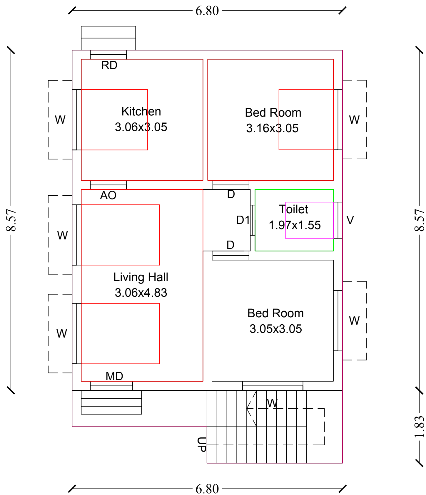
Ground Floor
