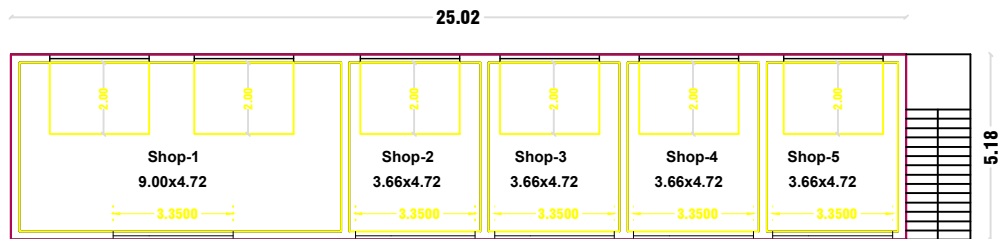
PRO. GROUND FLOOR PLAN
