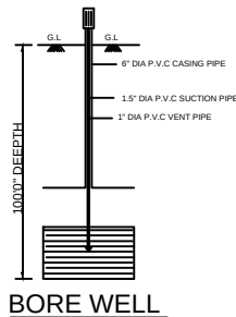
BORE WELL
