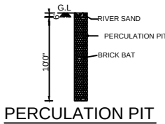
PERCOLATION PIT
