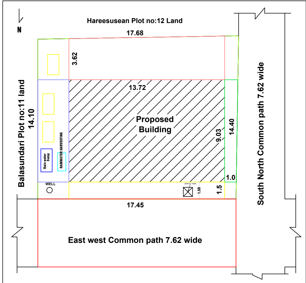
SITE PLAN CUM KEYPLAN
