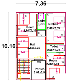
GROUND FLOOR F
