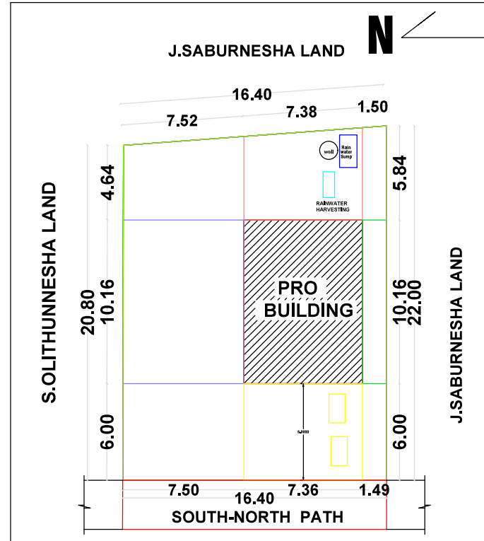
SITE PLAN & KEY PLAN (1:100)
