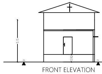
FRONT ELEVATION
