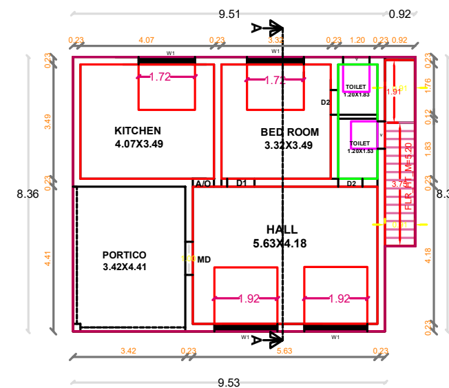
GROUND FLOOR PLAN PROPOSED
