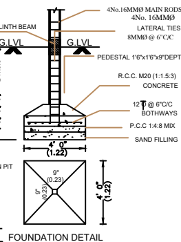
FOUNDATION DETAIL
