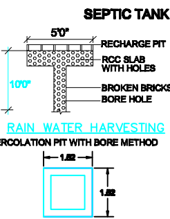
RAIN WATER HARVESTING PLAN
