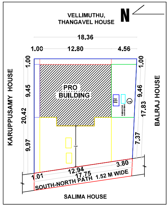
LOCATION & SITE PLAN
