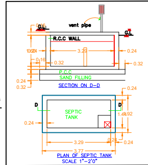
PLAN OF SEPTIC TANK SCALE 1"=2'0"
