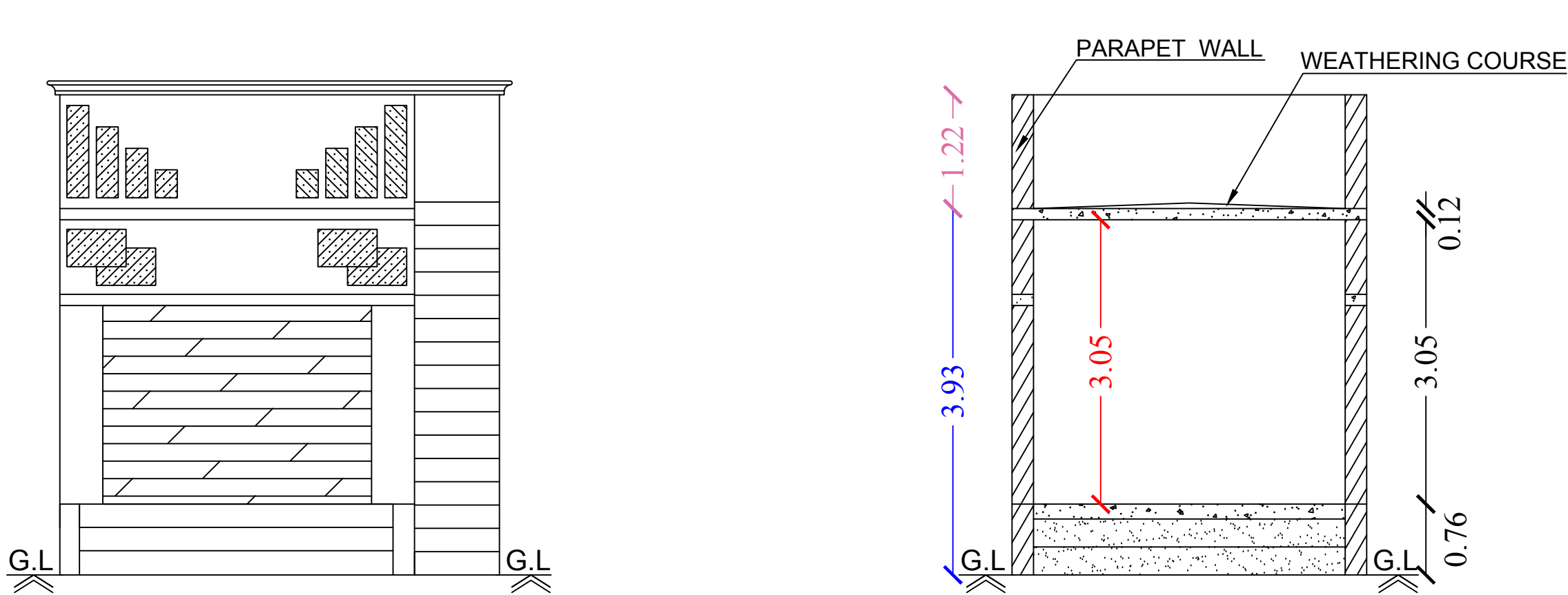
Front Elevation
