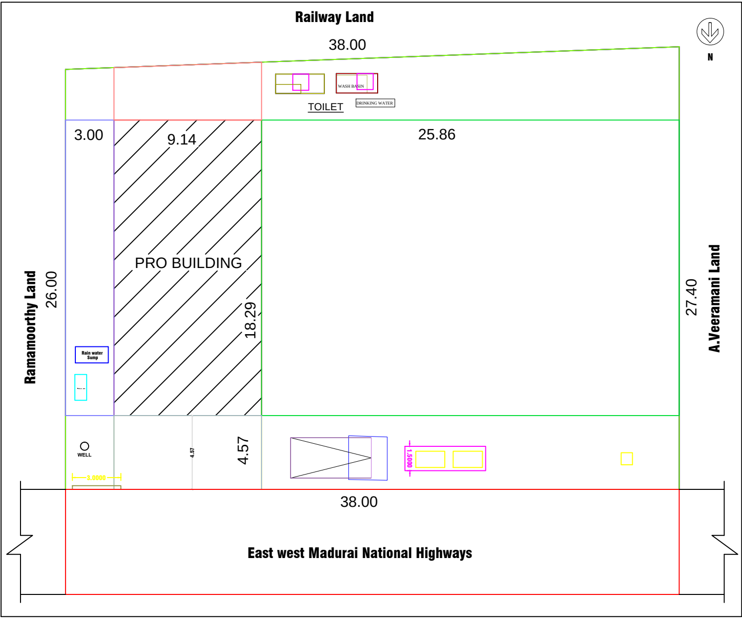
SITE PLAN & KEY PLAN
