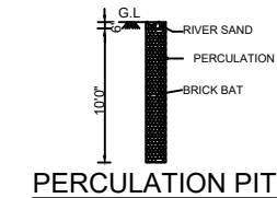
PERCOLATION PIT
