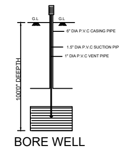
BORE WELL
