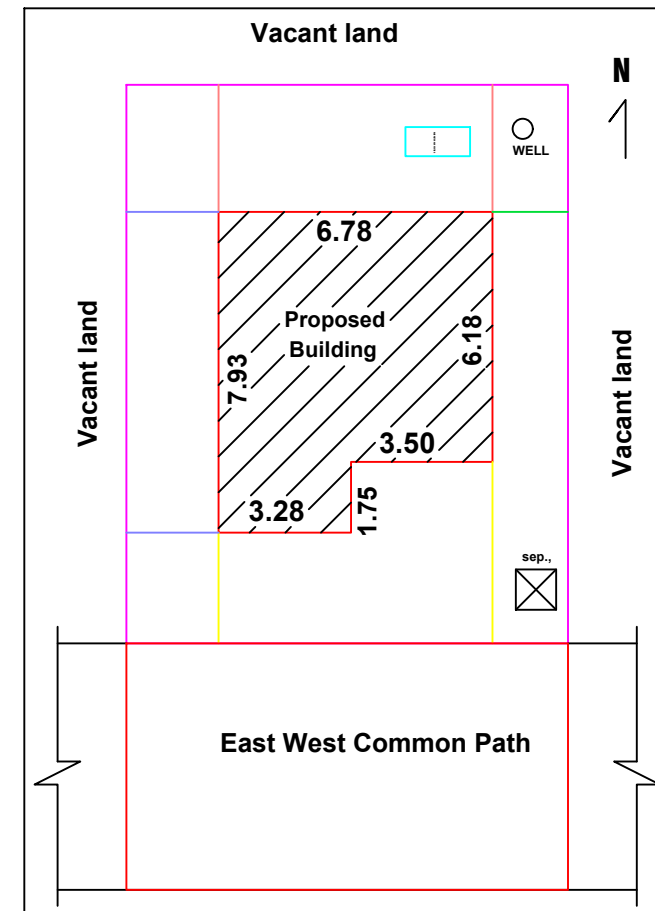
SITE PLAN CUM KEYPLAN
