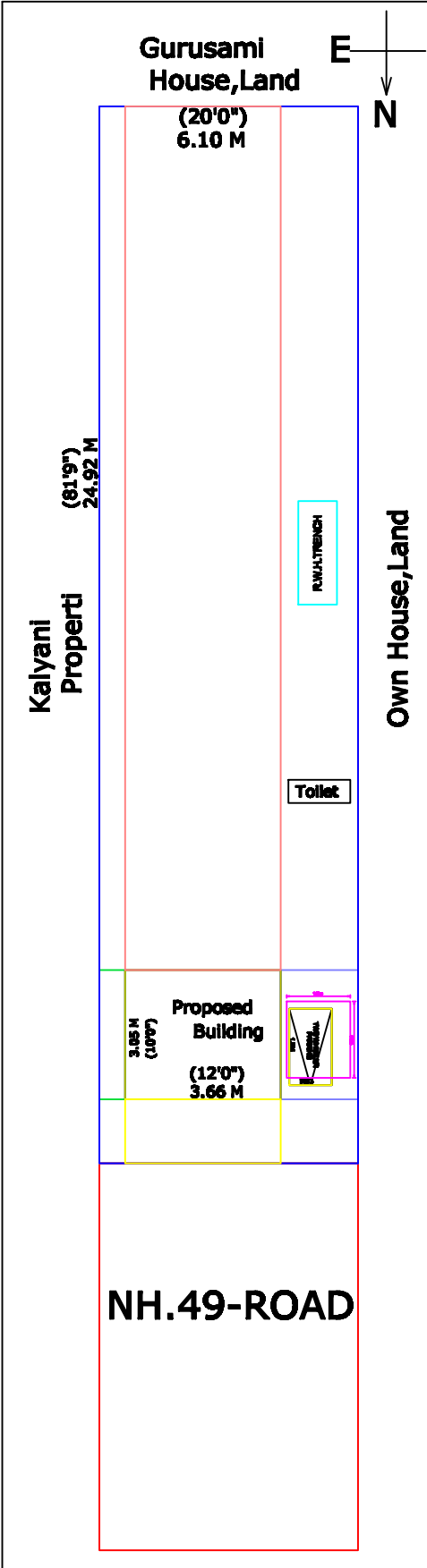
SITE PLAN
