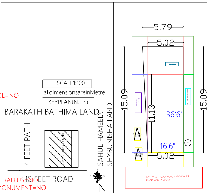
SITE PLAN CUM GROUND FLOOR & FIRST FLOOR PLAN
