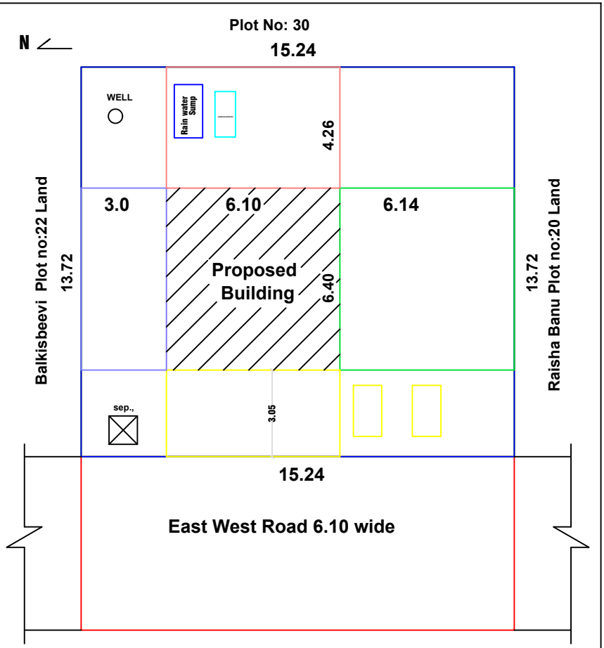
SITE PLAN CUM KEYPLAN
