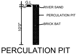
PERCOLATION PIT
