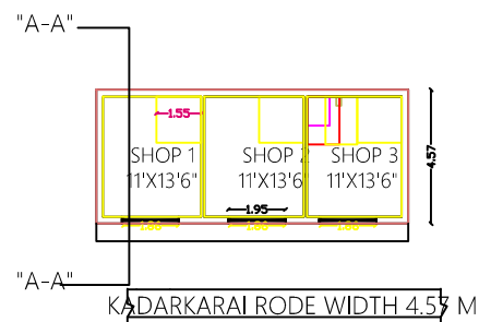
SITE PLAN CUM GROUND FLOOR PLAN
