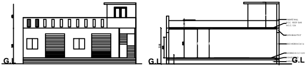
FRONT ELEVATION
