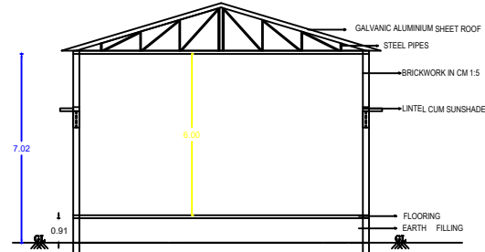
SECTION ON-AB
