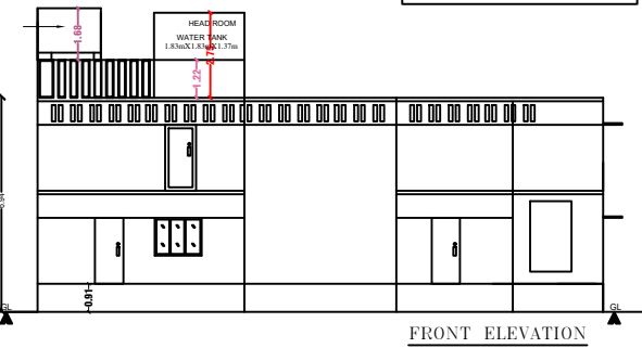
FRONT ELEVATION
