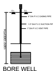
BORE WELL
