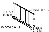
STAIRCASE DETAILS
