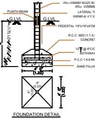
FOUNDATION DETAIL
