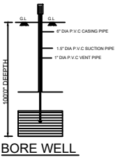
BORE WELL
