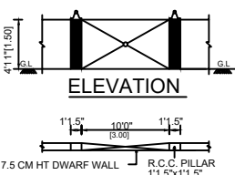
COMPOUND WALL PLAN
