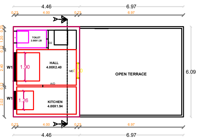
FIRST FLOOR PLAN PROPOSED
