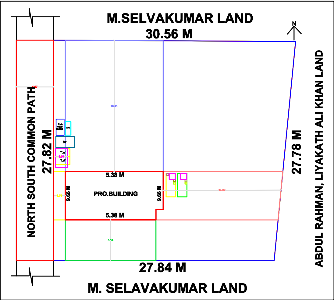
SITE PLAN
