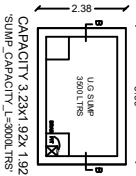
PLAN OF SWMP
