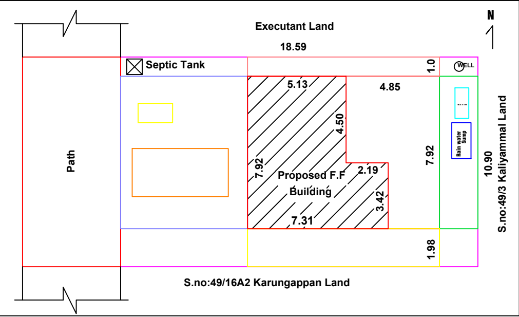
SITE PLAN CUM KEYPLAN
