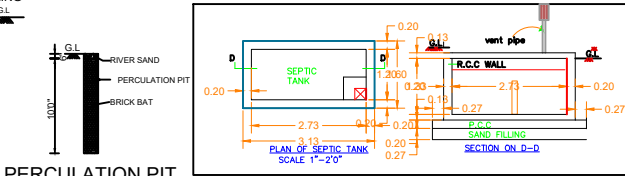
PERCOLATION PIT
