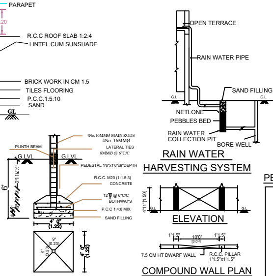
FOUNDATION DETAIL
